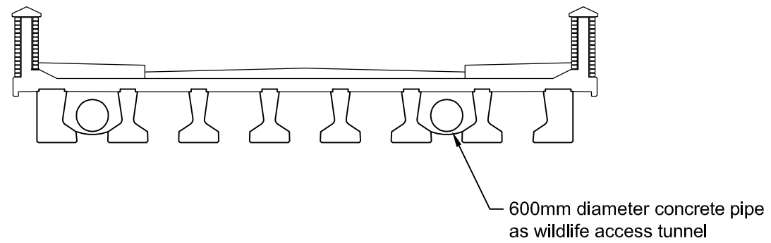
SECTION A-A TYPICAL DECK CROSS SECTION
